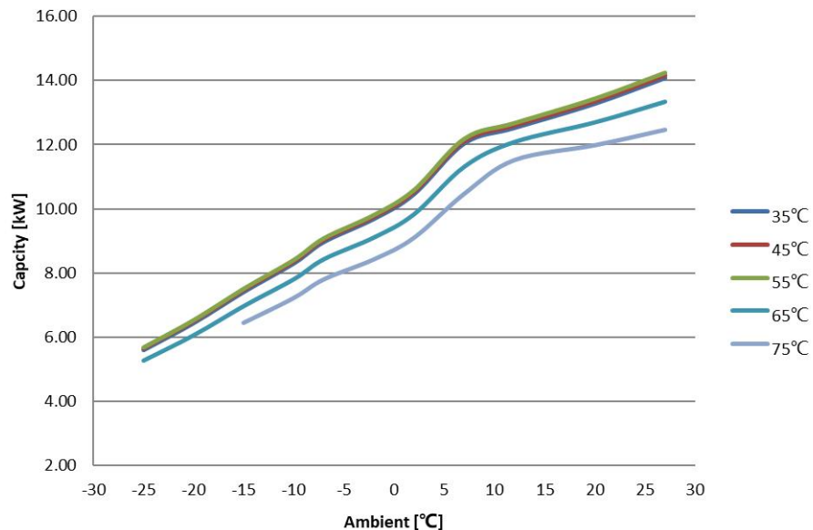
12kW Rated Heating Capacity Curve
