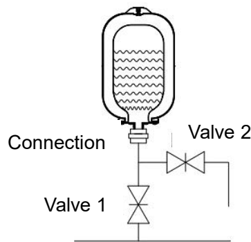
Expansion tank installation schematic
