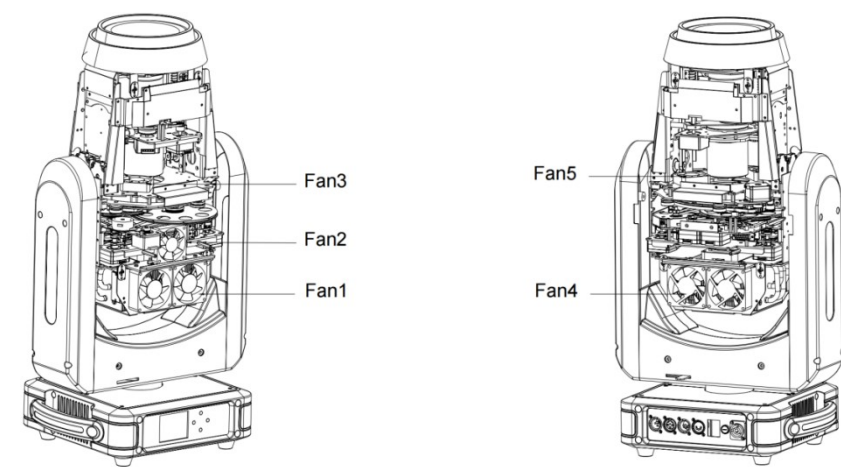
10.4 Lighting fan distribution diagram
