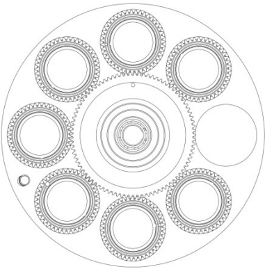
Rotating gobo (Fig.6.2-2)
