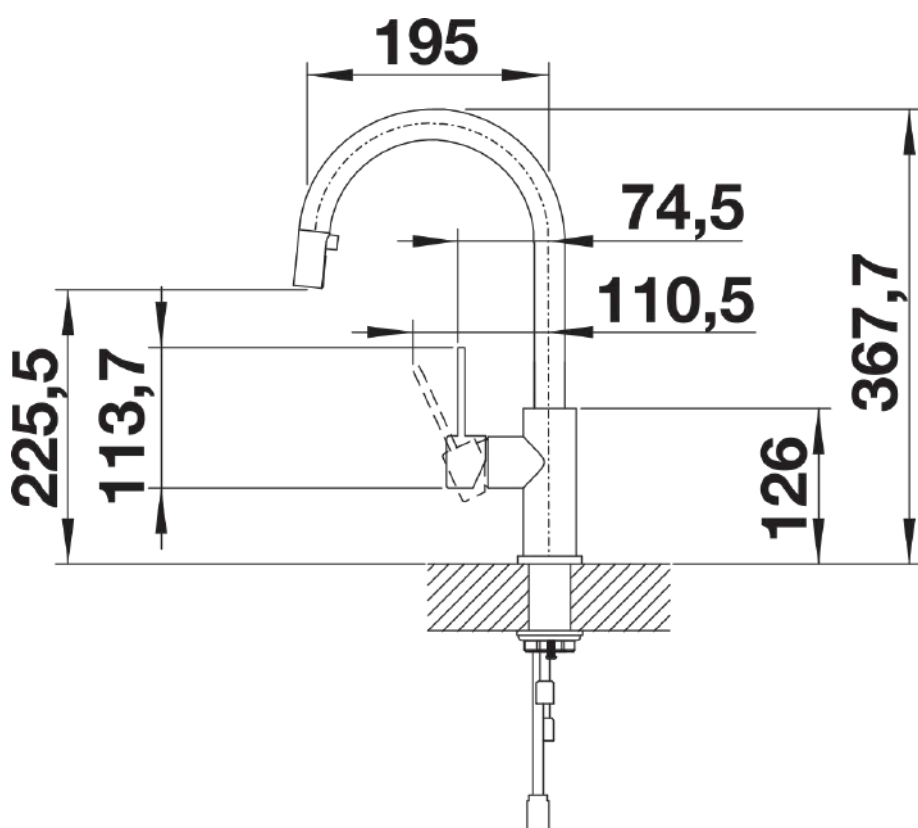
Side view
