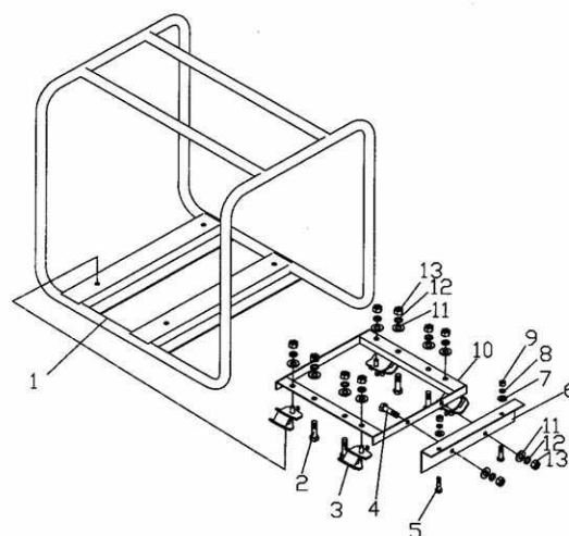
(3) Housing Assembly (KDP30-03000)
