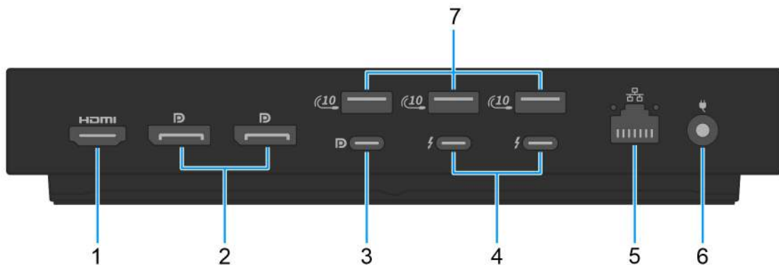
Figure 5. Back view
