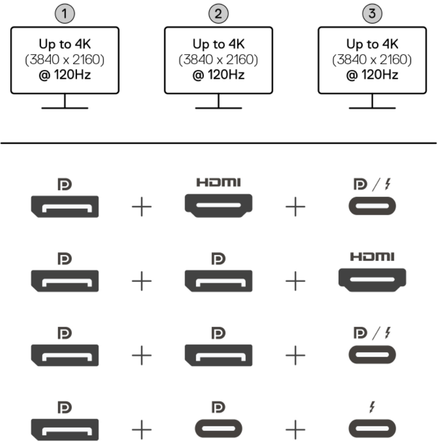
Figure 8. Triple-display setup
