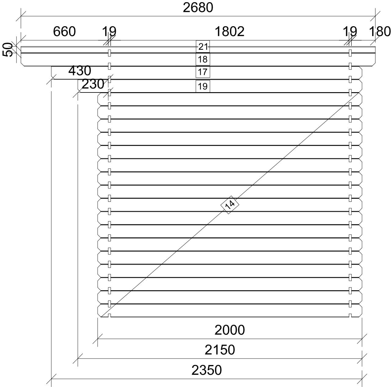
Arad 19mm F-4
