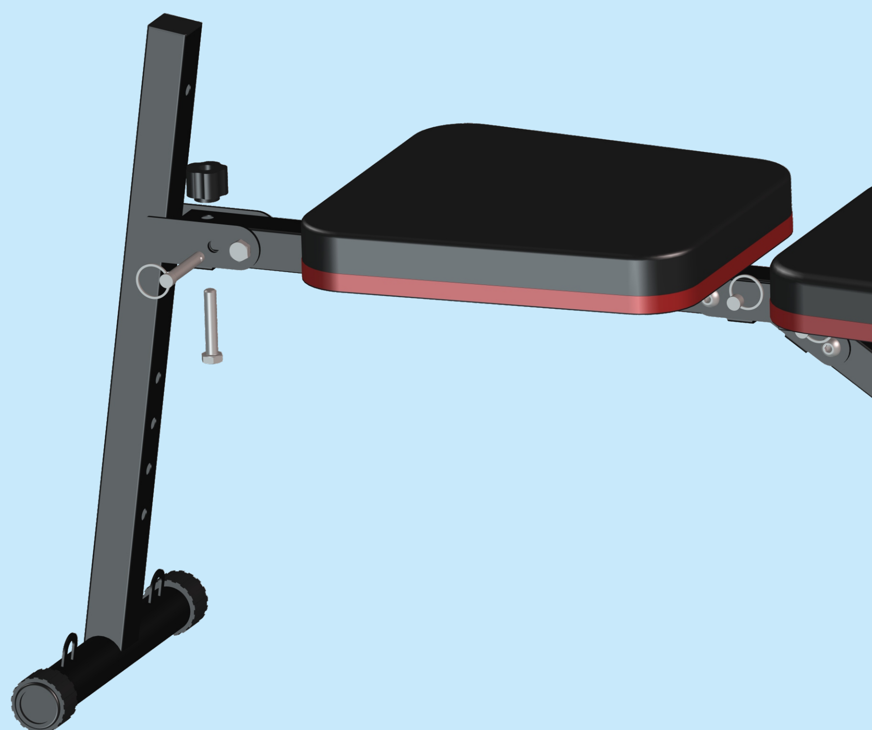
B、 Open the T-frame, and secure it with a ring pin(7) and hex bolt and plum nut.
