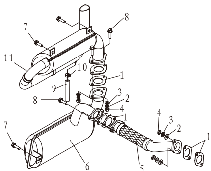
(8) Muffler Assembly
