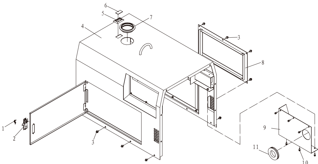
(5) Casing Unit
