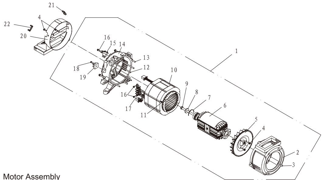
(2) Motor Assembly
