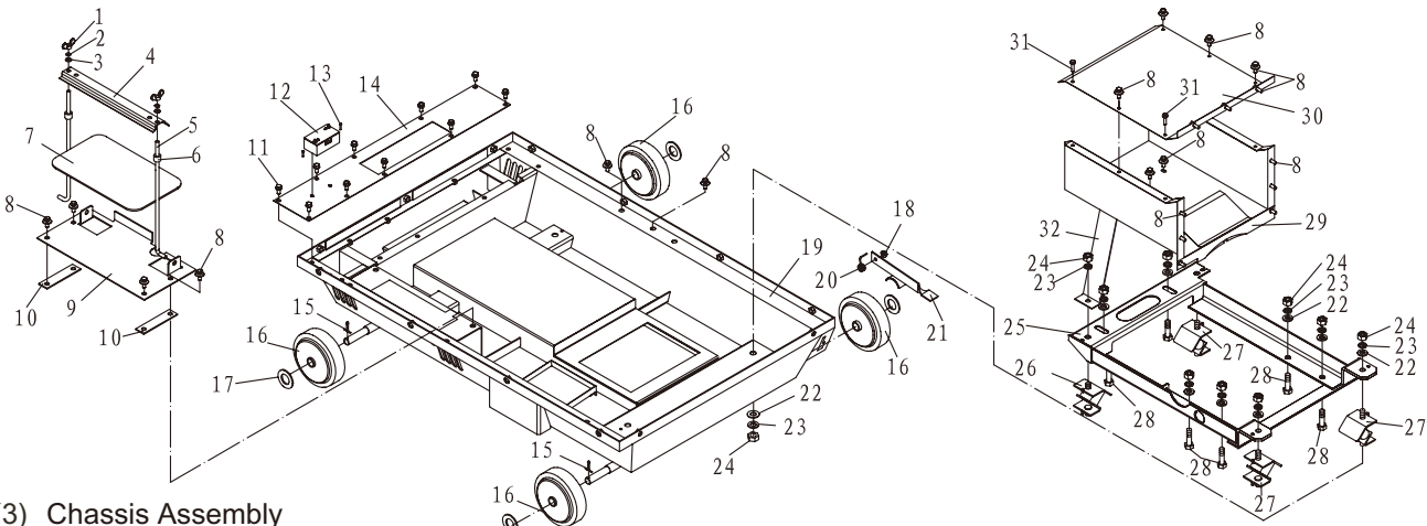
(3) Chassis Assembly
