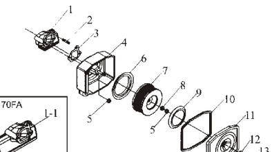
(7) Air Intake System (KM168F-07000)
