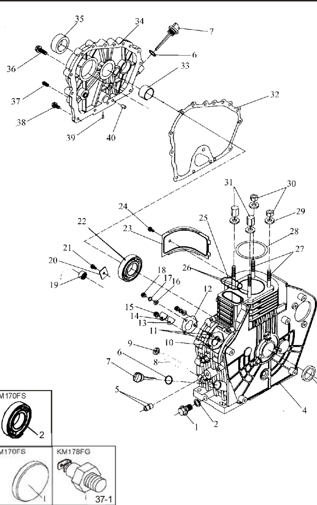
(1) Cylinder Block Assem. (KM170F-01000)
