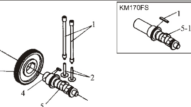
(6) Camshaft (KM168F-06000)
