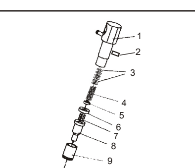
(8) Fuel Injection Valve Assem. (KM168F-13000)
