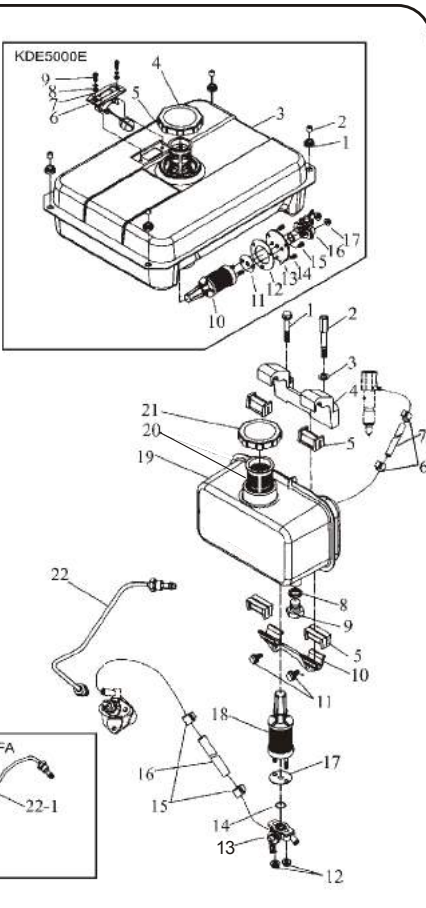
(11) Fuel System (KM168F-10000)
