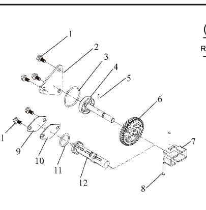
(10) Lubricating System (KM168F-09000)
