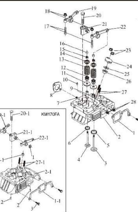
(2) Cylinder Head Assem. (KM168F-02000)
