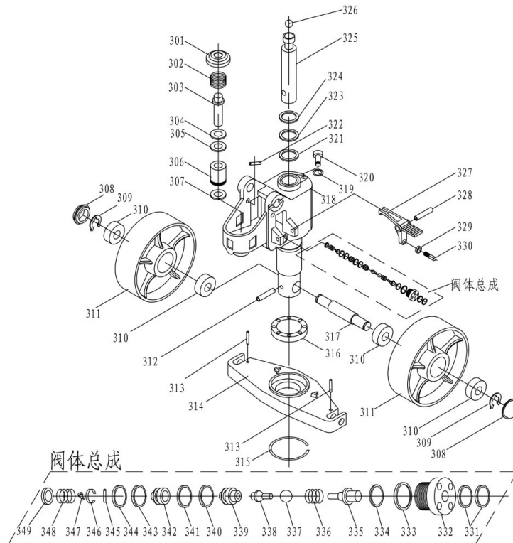
7-3 AC Oil Pump Assembly Drawing Oil Pump Part List
