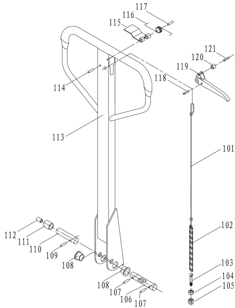
7-1 AC Handle Assembly Drawing
