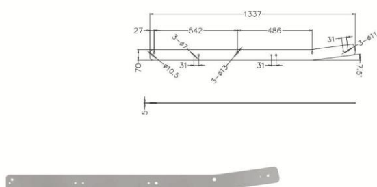
CONNECT PLATE-3 LT215L
