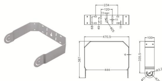
U TYPE BRACKET LT215
