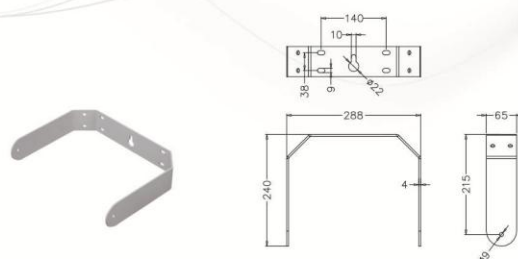
U TYPE BRACKET LT208
