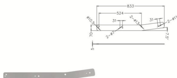
CONNECT PLATE-2 LT215L
