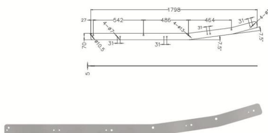
CONNECT PLATE-4 LT215L
