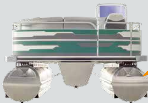
Boat hulls are made of marine grade aluminum alloy EN AW5083-H111. At the stern of the hulls very convenient built-in steps
