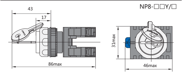
Dimension (mm)
