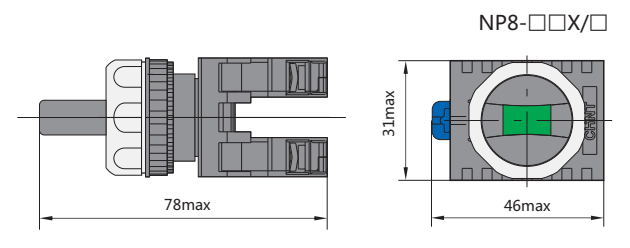
Dimension (mm)
