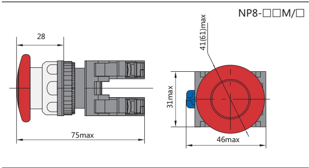
Dimension (mm)
