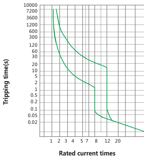
Fig.3 NM1-63(40~63), NM1-125(40~125) Characteristic Curve
