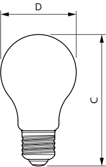
Bulb A60 6-60W 600lm 3000K E27 ND CL
