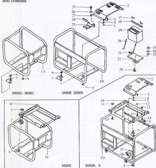
<B> KDE2500 KDE3500 KDE5500 Parts drawing of frame, trimboard and chassis
