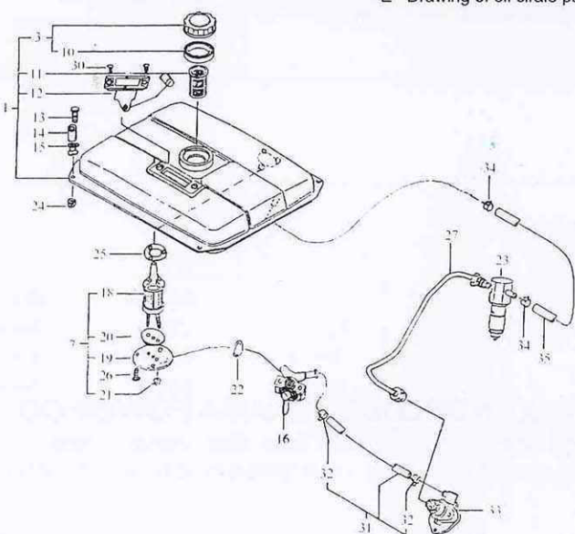
&lt;E&gt; Drawing of oil ciraie parts
