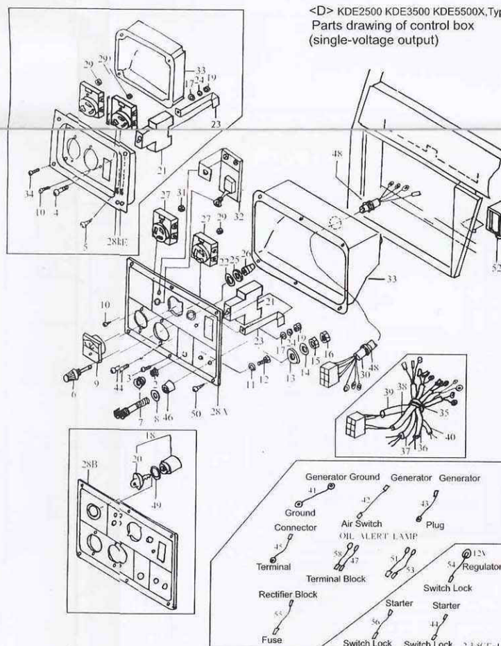
C.D Parts list of control box
