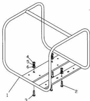
(3) Housing Assembly (KGP20-03000)
