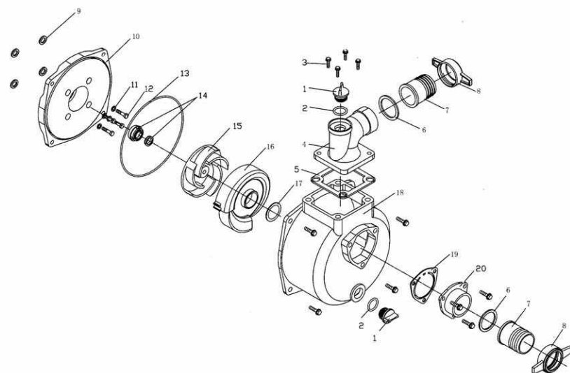
(2) 2" Pump Assembly (50KBZ-01000C)
