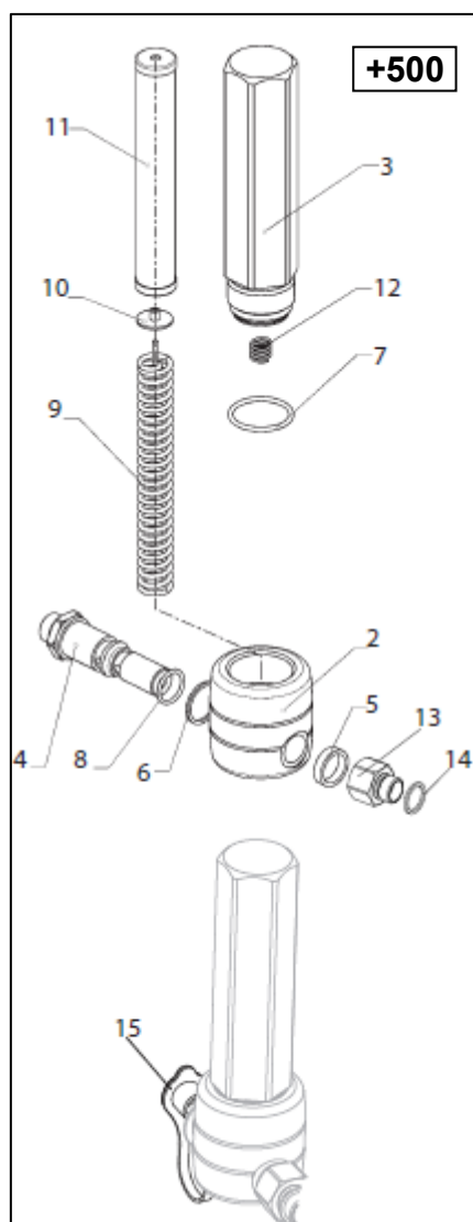
parts diagram high-pressure filter
